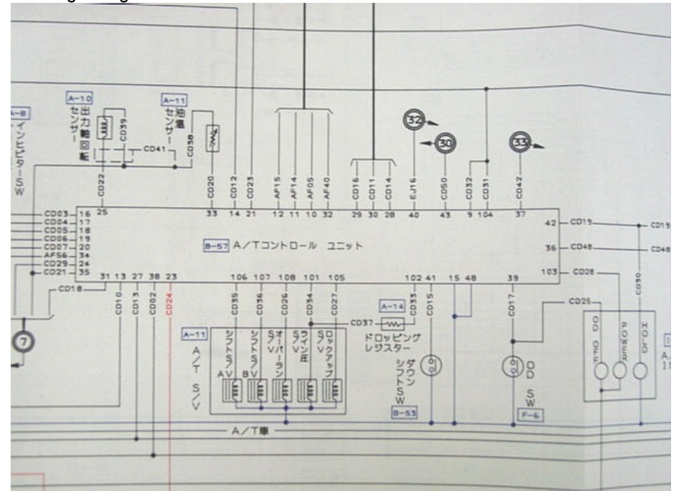
Wiring diagram
